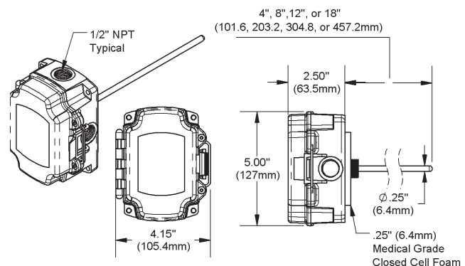
Wireless Duct Temperature unit in a BAPI-Box (BB) Enclosure
